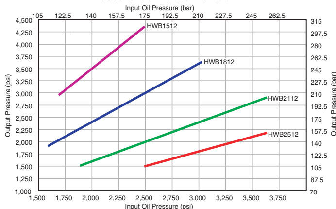
Pressure Conversion Chart
