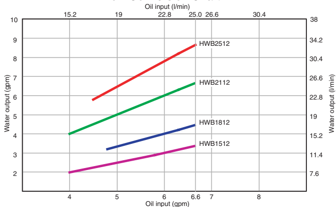
Flow Conversion Chart
